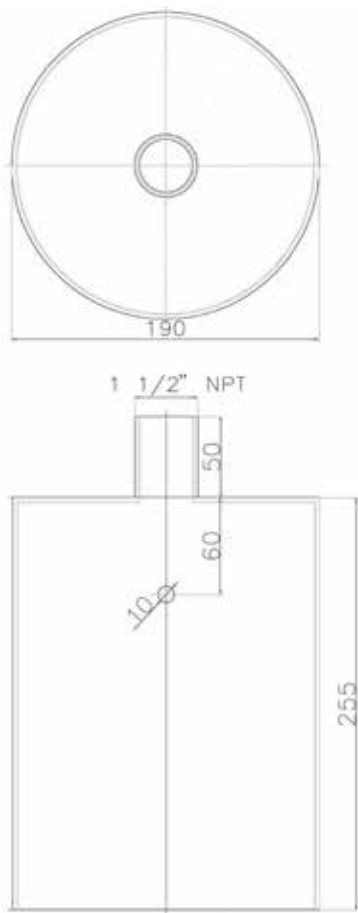
Dimensions: OD-A
